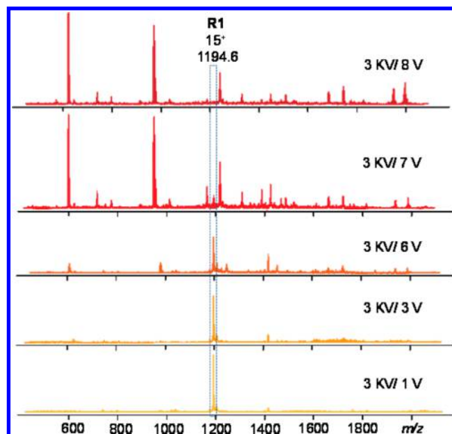
Figure 3. Gradient tandem-mass spectrometry (gMS 2 ) of R1 at m/z 1194.6 (15 + ) with different collision energy.
