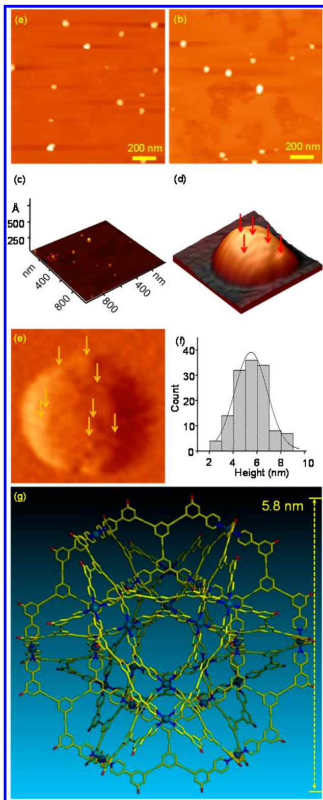
Figure 9. (a,b) AFM images of S with \text{BF}_4^- as counterion. (c) 3D AFM image. (d) Zoom-in 3D image of the dot labeled by red circle. (e) Amplitude image of the dot labeled by red circle. (f) Statistical height histogram of AFM for 129 dots. (g) Representative energy-minimized structure of S from molecular modeling. The long alkyl chains are omitted for clarity in the molecular modeling.
