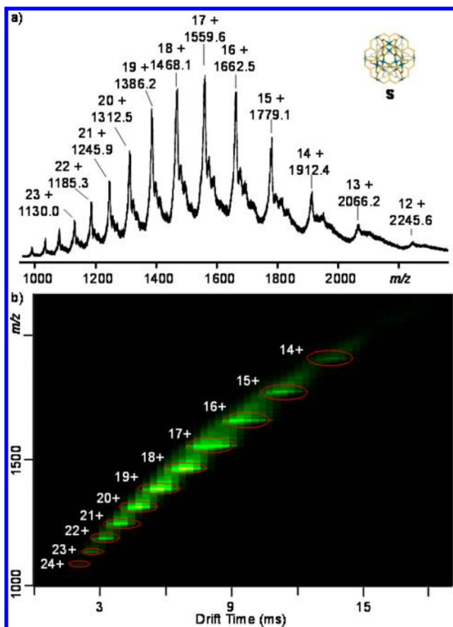
Figure 6. (a) ESI-MS and 2D ESI-IM-MS plot ( m/z vs drift time) of S with \text{BF}_4^- as counterion. (b) The charge states of intact assemblies are marked.
