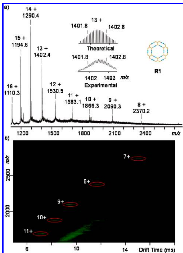
Figure 2. (a) ESI-MS of R1, with an inset showing the theoretical and experimental isotopic patterns of the 13 + signal. (b) 2D ESI-IM-MS plot ( m/z vs drift time) of R1. The charge states of intact assemblies are marked.
