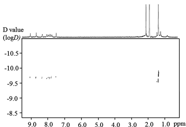
Fig. 3 2D-DOSY NMR (500 MHz) of [\text{Cd}_{12}\text{L}_{28}] in \text{CD}_3\text{CN} .
